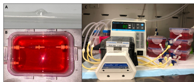
Figure 1 Silicone aneurysm tubes and bioreactor system configuration. Silicone aneurysm tubes were 43 mm in length, with 4.0 mm internal diameter, and incorporated aneurysms with a 2.4 mm neck and 3.1 mm height (A). Silicone aneurysm tubes were coated with fibronectin then placed in individual bioreactor chambers prior to cell deposition (B). Individual bioreactor systems were connected to media reservoirs, placed on peristaltic pumps, and run at 37°C and 5% CO 2 , before and after cell deposition (C).
